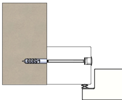
Blockrahmen 100 mm x 80 mm
